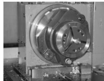
Rotary table
