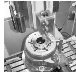
Shaping machine
